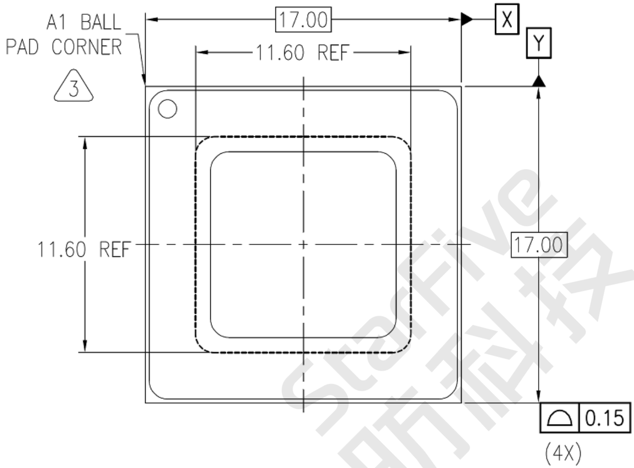
Figure 7-2 Package Top View
