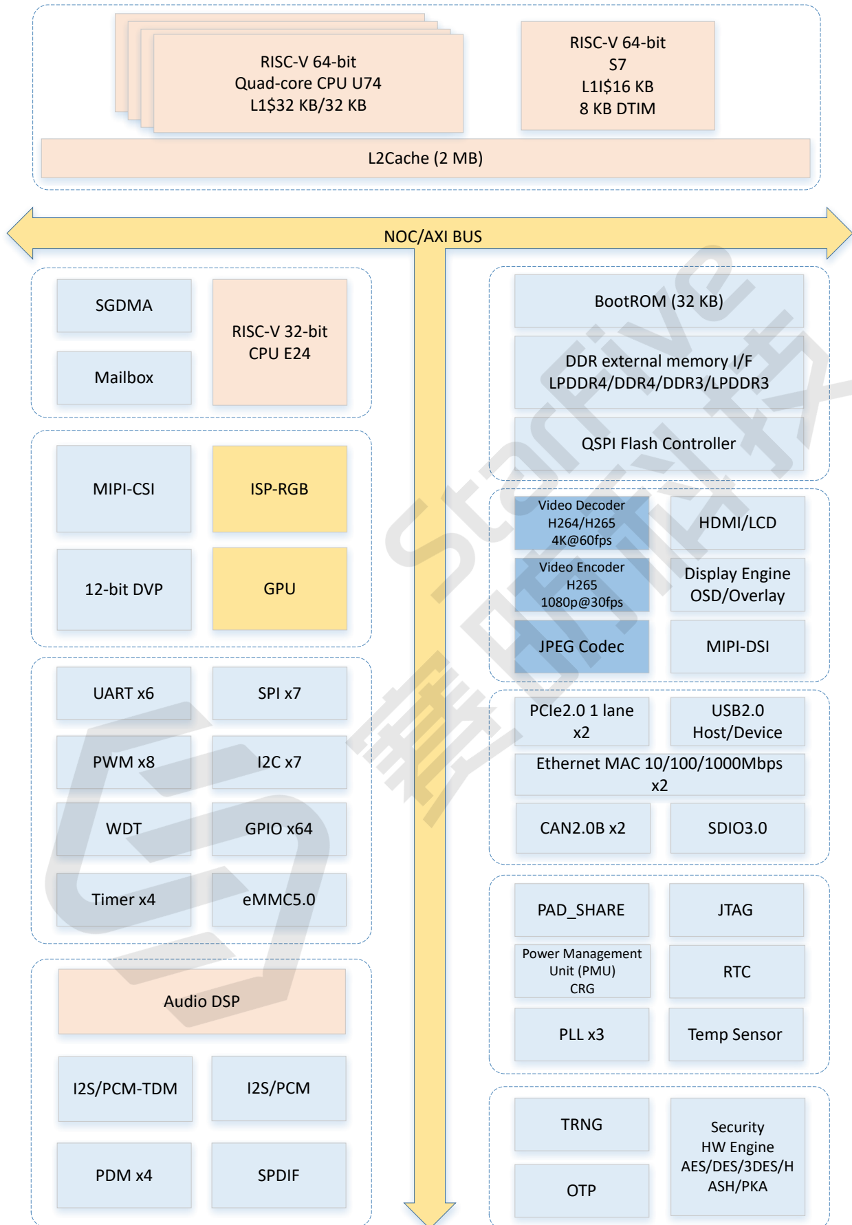
Figure 1-1 Block Diagram
